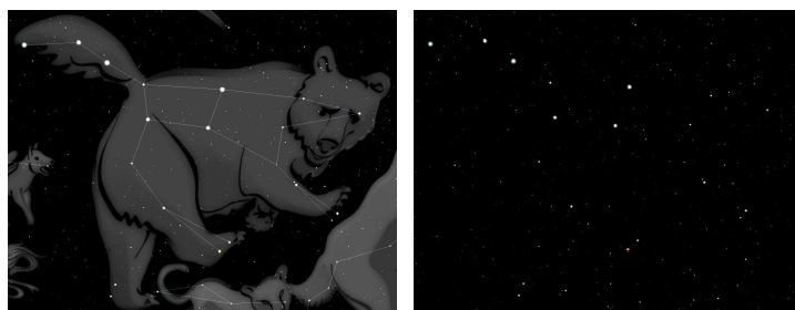
Figura 2: The constellation of Ursa Major.
